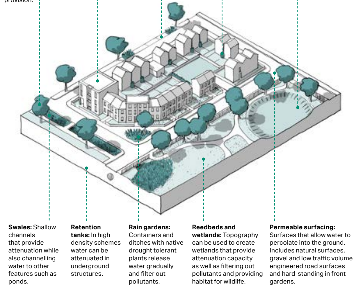
Figure 82: Sustainable drainage systems as set out in the National Model Design Code.
